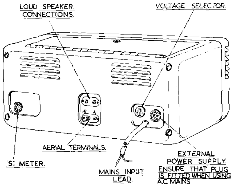
Fig. 4. Rear outline of Receiver, indicating external connections.
