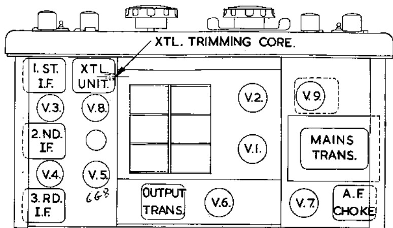
Fig. 5. Plan view in outline.
